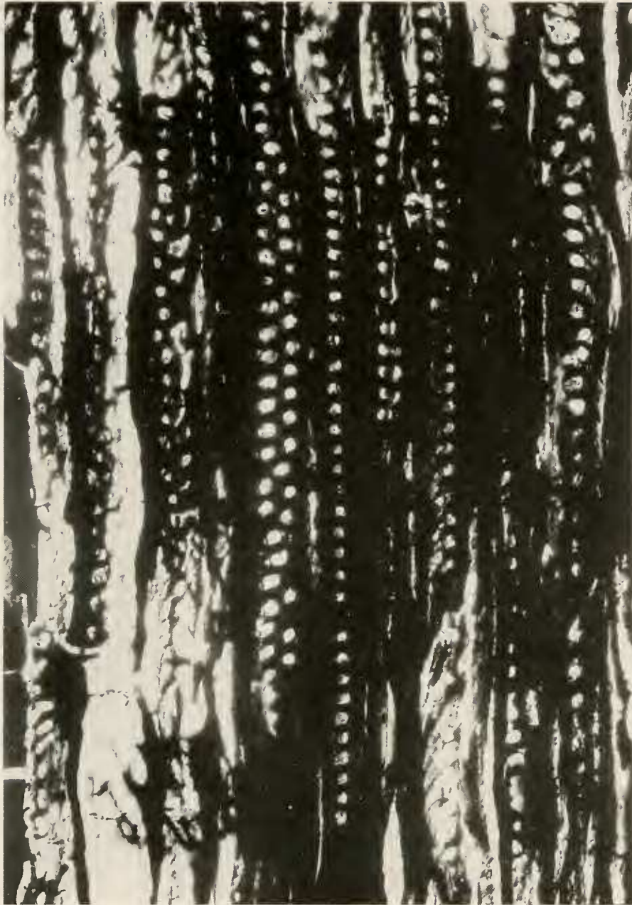
Fig. 20. Radial longitudinal section showing radial walls with uni- and biseriate rows of bordered pits. x 250.
